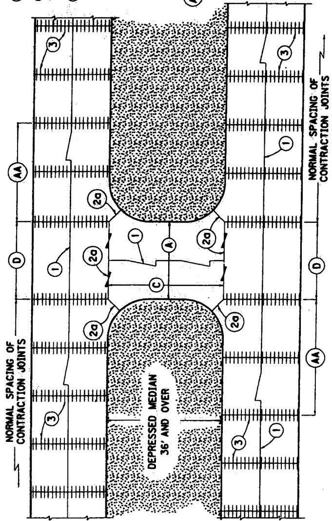
TYPICAL DIVIDED PAVEMENT WITH DEPRESSED MEDIAN AND CROSSOVER
