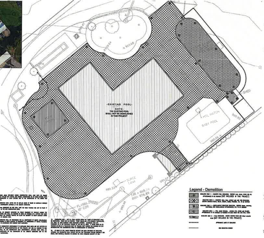
Site Plan - Demolition Site Photo 7/3/12
