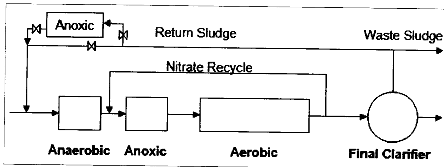
A 2 /O Process Schematic
