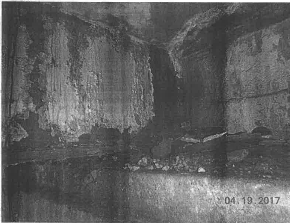
Beam end of beam #4 at abutment #2 has a 6" hole in the web near the LF with the bottom flange being severed at the bearing.
