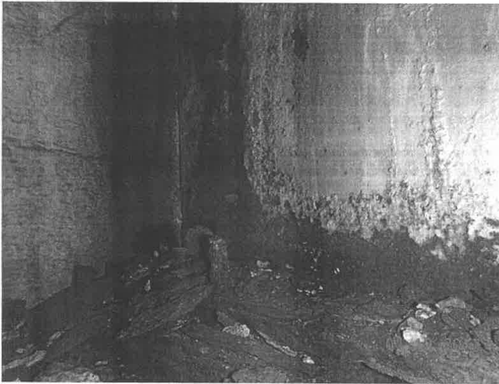
Beam end of beam #8 at abutment #2 has moderate section loss in the last 3' of beam
