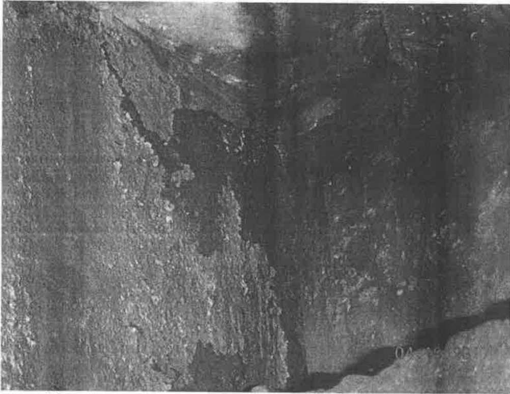
Beam end of beam #5 at abutment #1 has a 1"x1" hole in the web near the TF
