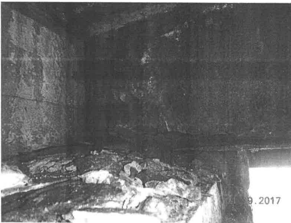
View of the beam end of beam #9 at abutment #2 has holes in the web in the last 19'
