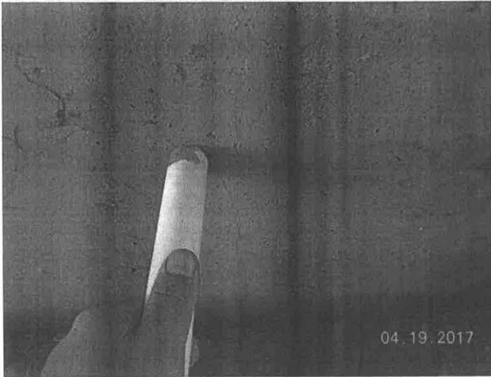
Typical view of the HL cracking in the LF of the box beams at the abutments,
