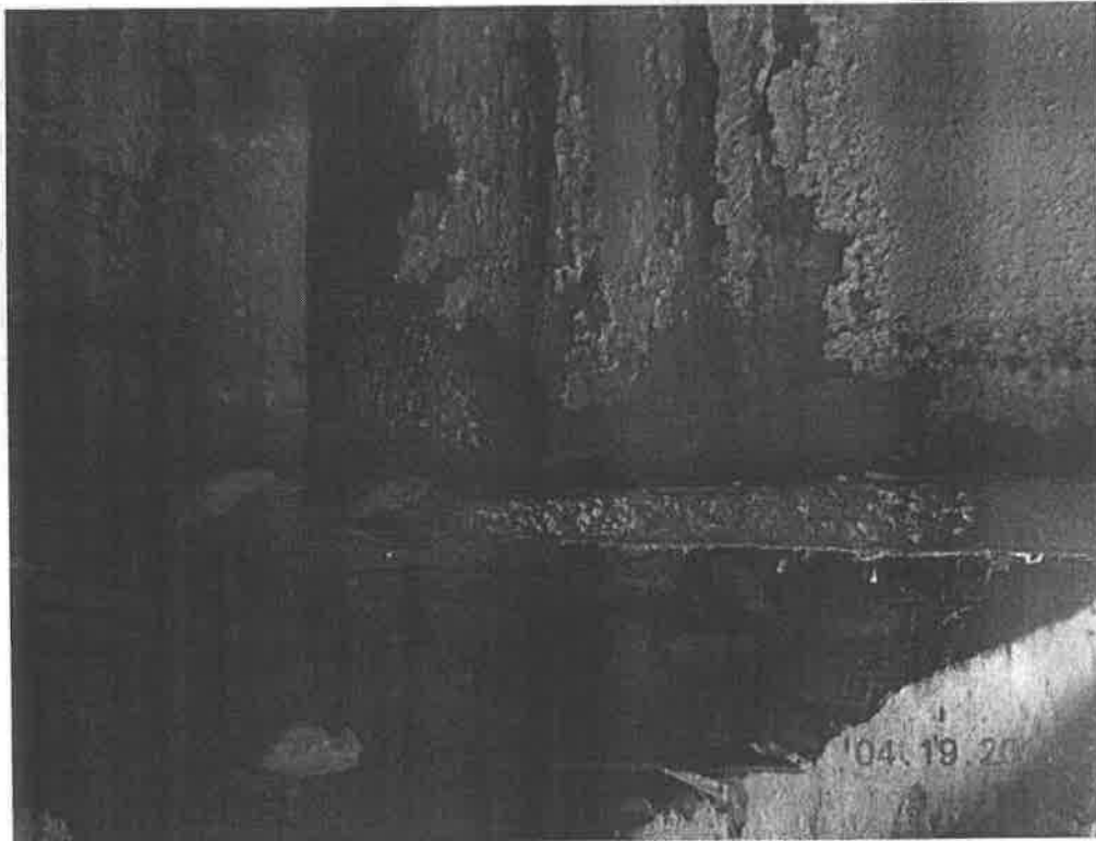
Beam end of beam #6 at abutment #2 section loss in the web (3') and LF 1/4" remaining at the face of the bearing
