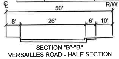
SECTION "B"-"B" VERSAILLES ROAD - HALF SECTION
