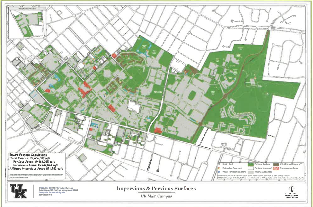
FIGURE 1 – UK MUNICIPAL SEPARATE STORM SEWER (MS4) MAP (FROM APPLICATION)
