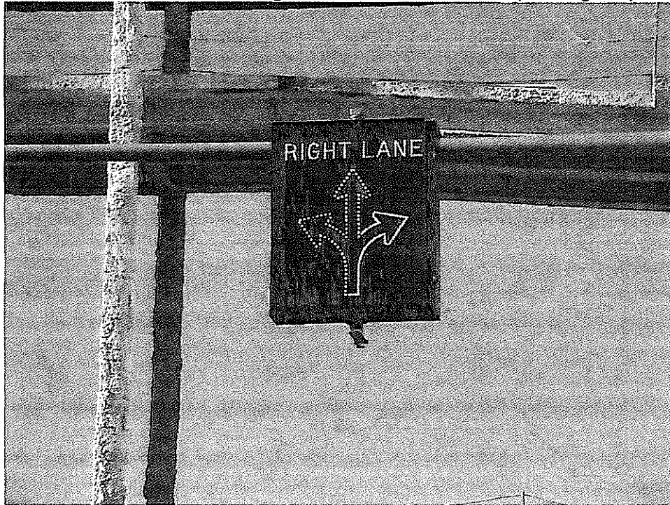
LED Lane Use Control Signal, 30-inch x 36-inch, #2 (Message #1)
