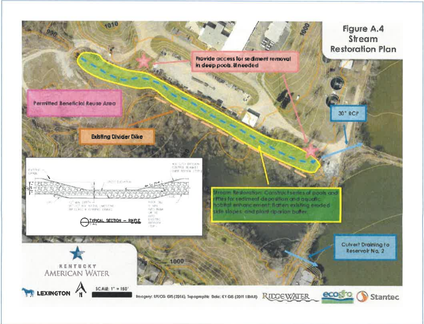
FIGURE 3 – PROJECT AREA/STREAM RESTORATION PLAN (FROM APPLICATION)
