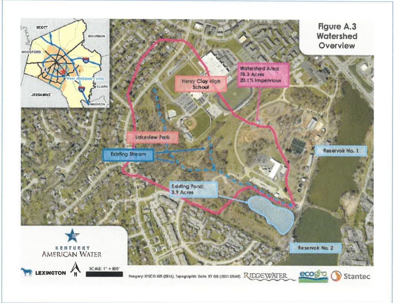
FIGURE 2 – KAWC WATERSHED OVERVIEW (FROM APPLICATION)
