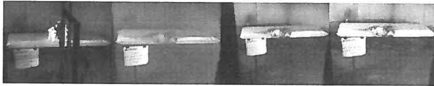
PHOTO(s) 2. Mattress During Testing to 16 CFR 1633
