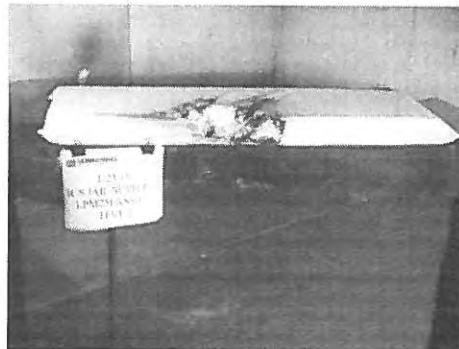
PHOTO 3. Mattress After Testing to 16 CFR 1633
