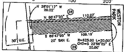
DETAIL OF 20' SANITARY EASEMENT TO BE RELEASED
