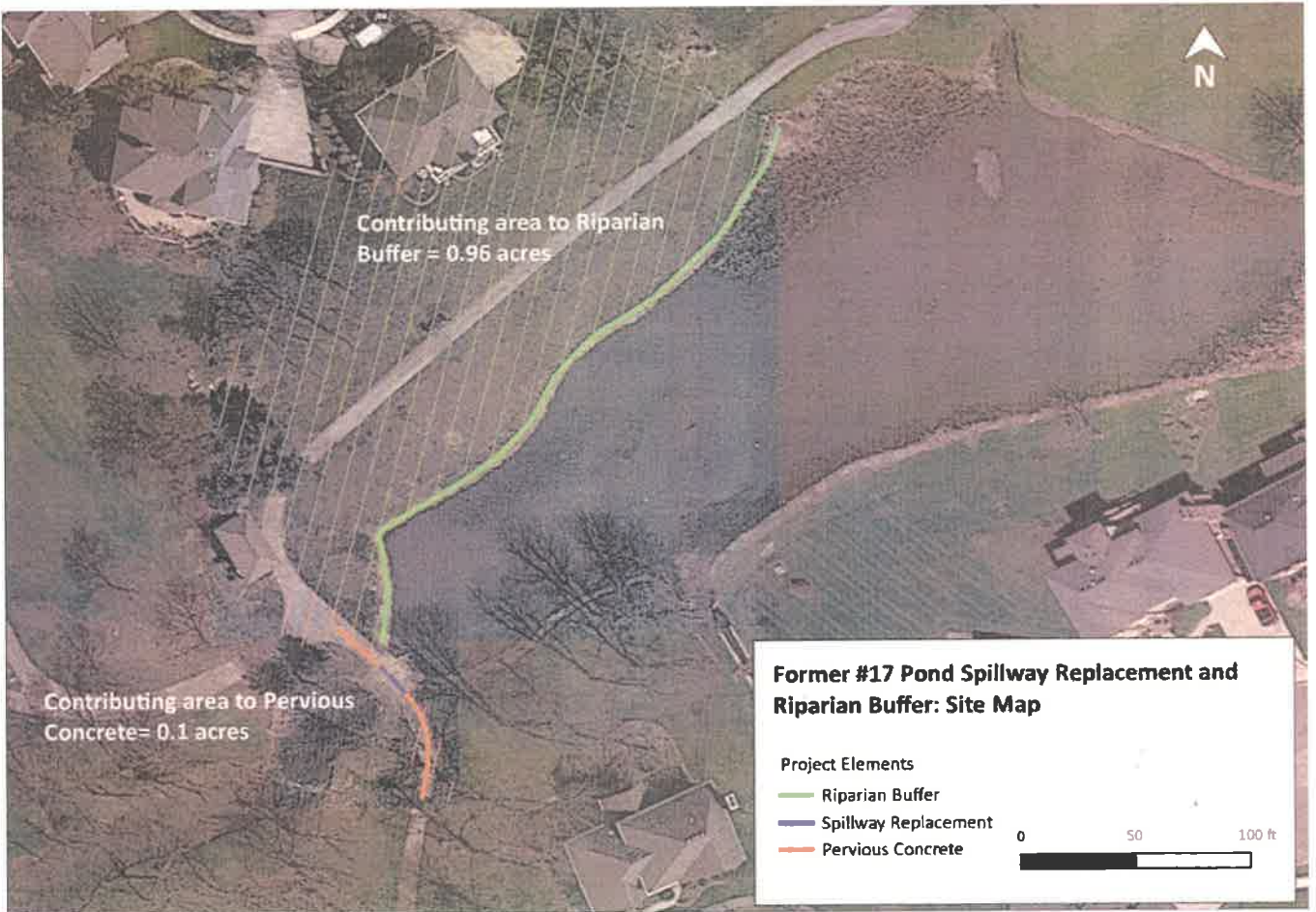
FIGURE 2 – DRAINAGE AREA OF PROPOSED FACILITIES (FROM APPLICATION)
