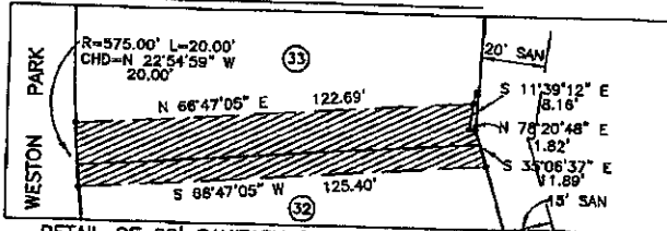
DETAIL OF 20' SANITARY SEWER EASEMENT TO BE RELEASED
