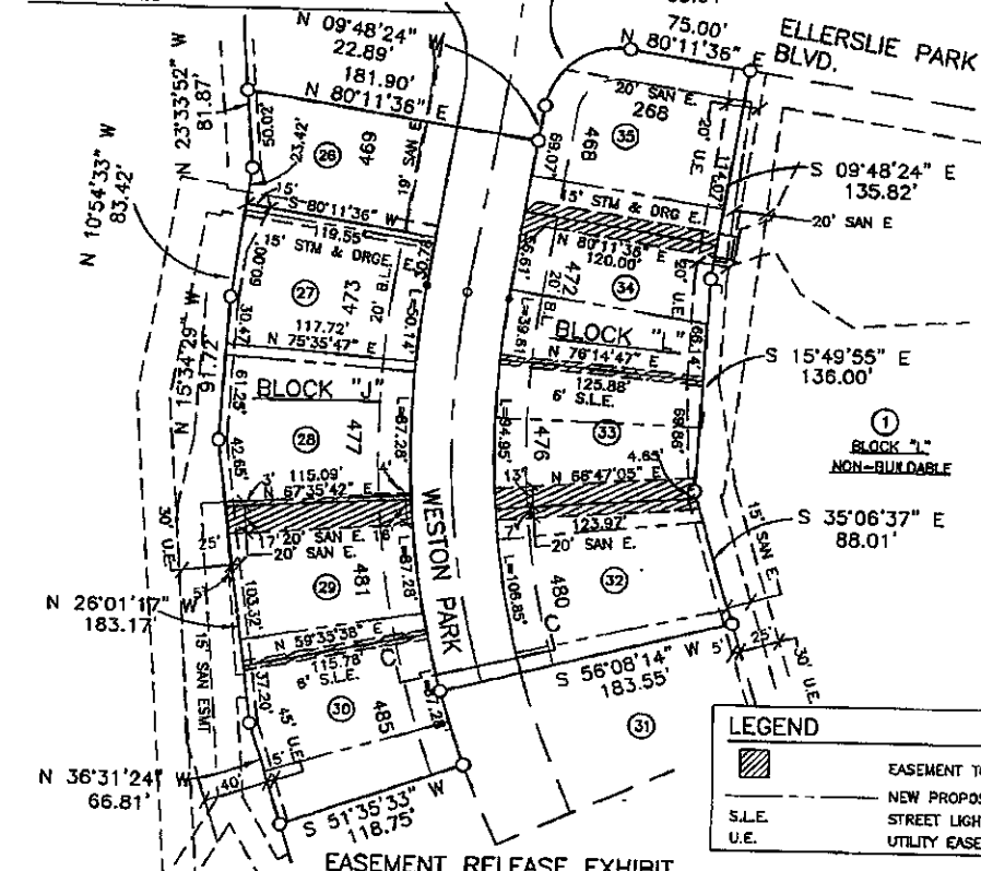
EASEMENT RELEASE EXHIBIT SCALE: 1"=100'
