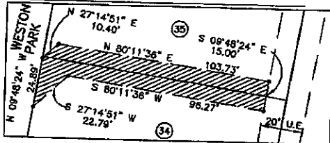
DETAIL OF 15' STORM & DRG. EASEMENT TO BE RELEASED
