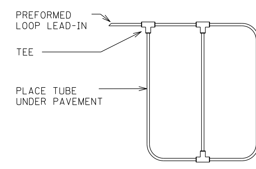
PREFORMED LOOP DIAGRAM
