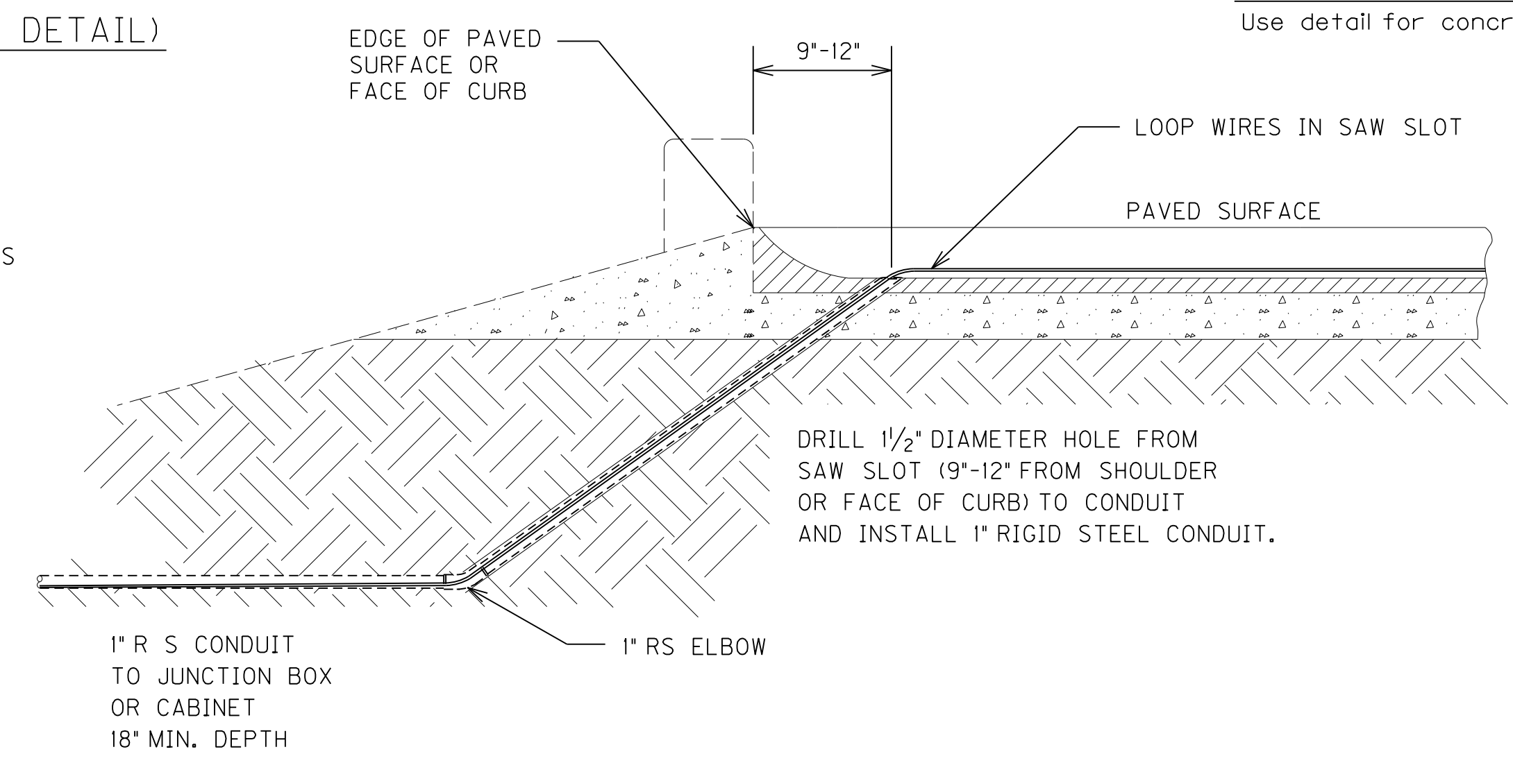
SAW SLOT EDGE OF PAVEMENT TRANSITION
