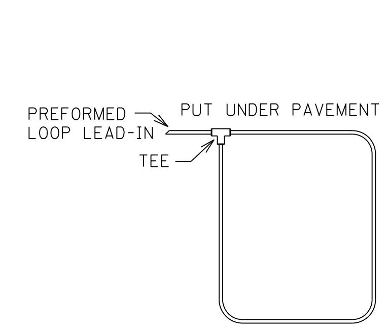
PREFORMED LOOP DIAGRAM
