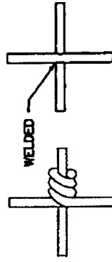
ALTERNATE METHODS OF SECURING VERTICAL STAY WIRE TO THE HORIZONTAL WIRE OF THE FABRIC.
