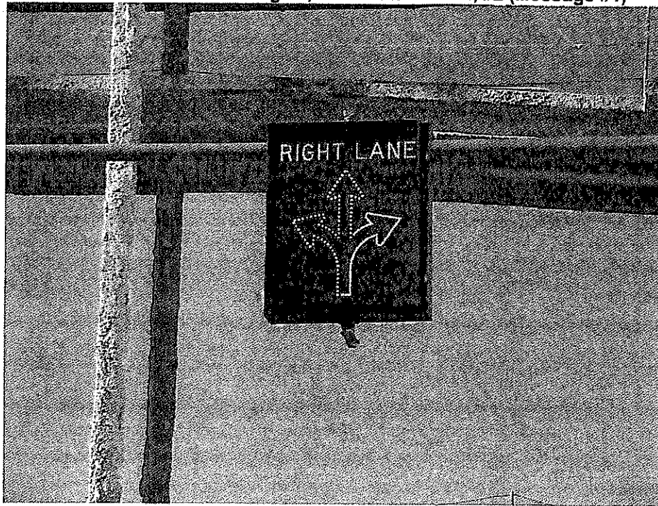
LED Lane Use Control Signal, 30-inch x 36-inch, #2 (Message #1)
