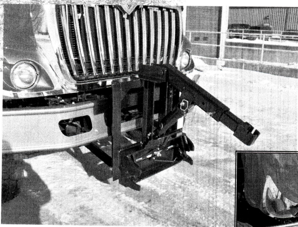
Shown with Quick Link Receiver, standard is 30-1/2" center push point.
