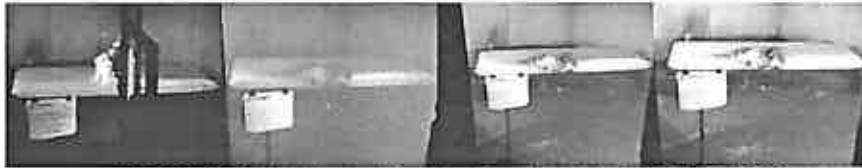
PHOTO(s) 2. Mattress During Testing to 16 CFR 1633
