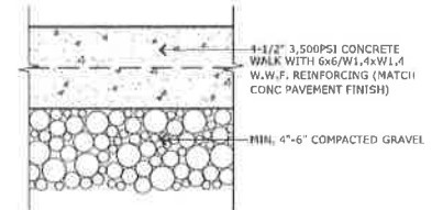
H LIGHT DUTY CONC SIDEWALK A.3 3' = 1'-0"
