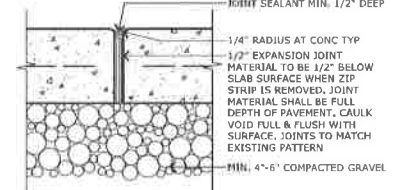
G LIGHT DUTY TYP EXPANSION JT A.3 3' = 1'-0"
