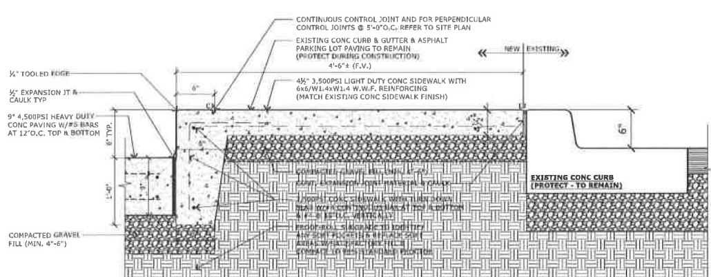
A LIGHT DUTY CONC SIDEWALK DETAIL A.3 SC: 1 1/2\"/>
