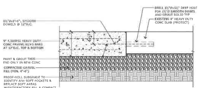
B HEAVY DUTY CONC CONSTRUCTION JT A.3 SC: 1 1/2\"/>
