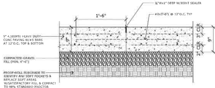
C HEAVY DUTY CONC CONSTRUCTION JT A.3 SC: 1 1/2\"/>
