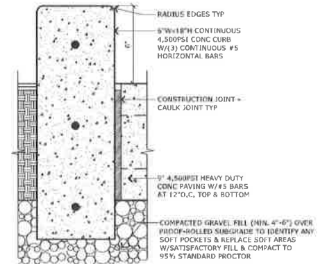
I TYPICAL CONC HEADER CURB A.3 3' = 1'-0"
