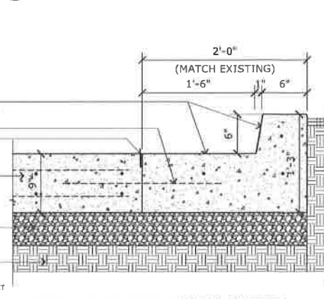
E HEAVY DUTY CONC CURB & GUTTER A.3 SC: 1 1/2\"/>
