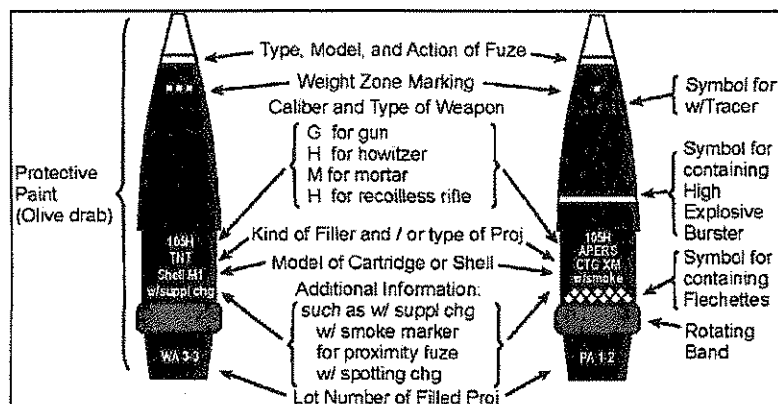
Figure 8.1: Ammunition markings
