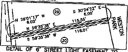
DETAIL OF 6' STREET LIGHT EASEMENT TO BE RELEASED
