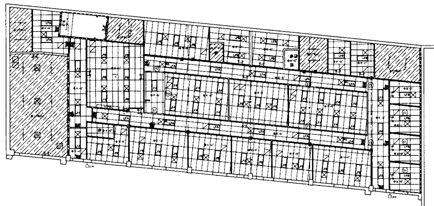
LOWER LEVEL REFLECTED CEILING PLAN SCALE: 1/8" = 1'-0"
