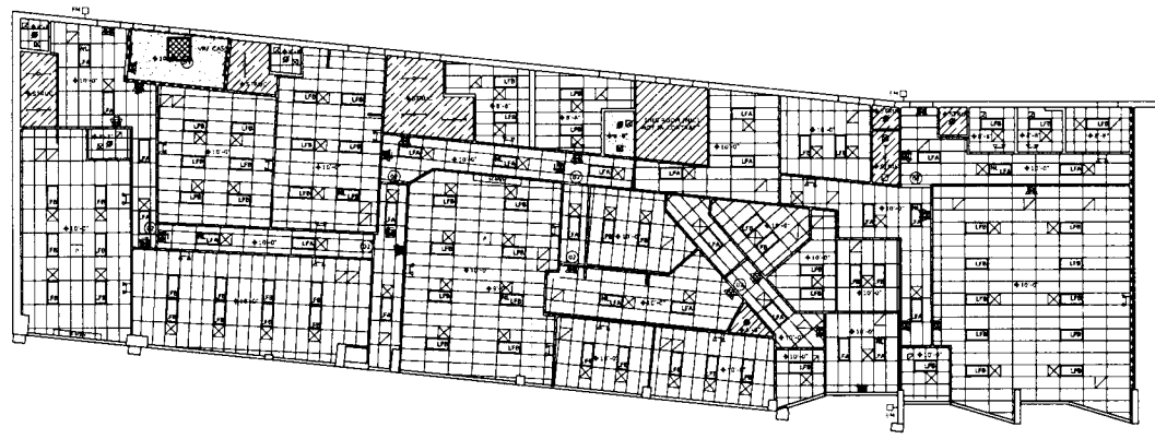
UPPER LEVEL REFLECTED CEILING PLAN SCALE: 1/8" = 1'-0"
