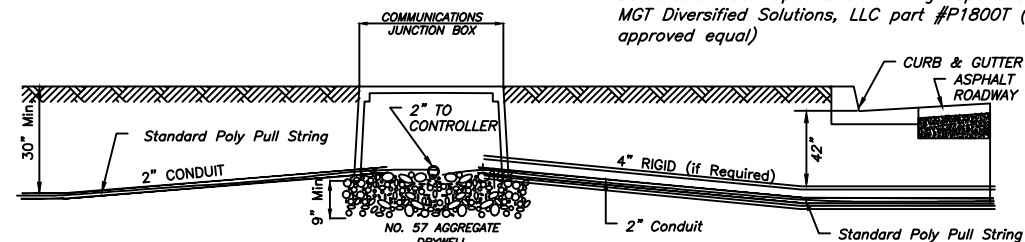
COMMUNICATIONS CONDUIT - STANDARD INSTALLATION - PROFILE
