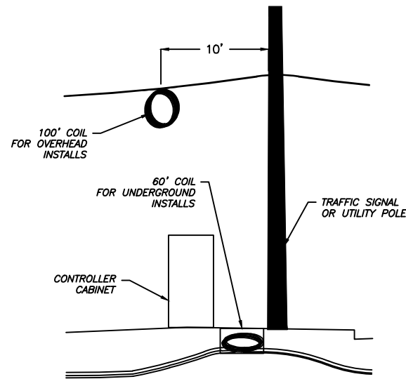
TYPICAL SLACK LOOP ARRANGMENT AT EACH TRAFFIC SIGNAL
