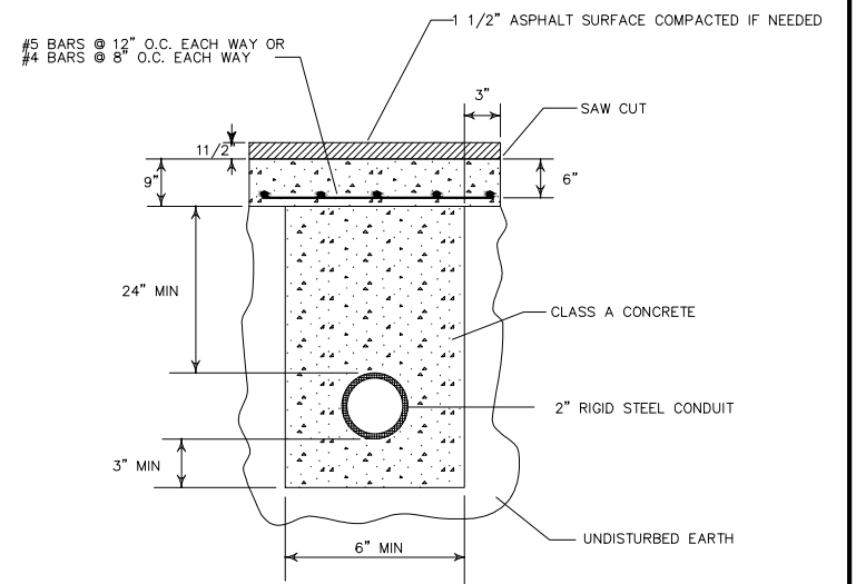
METHOD FOR REPAIRING OPEN CUT PAVEMENT
