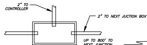
STANDARD INSTALLATION - PLAN VIEW
