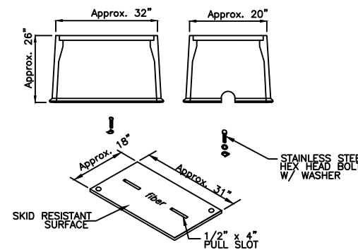
COMMUNICATIONS JUNCTION BOX - TRAFFIC BEARING, FIBER-OPTIC
