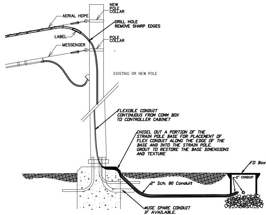
FIBER TO EXISTING STRAIN POLE
