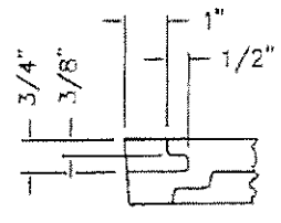
PICKHOLE DETAIL QUARTER SCALE
