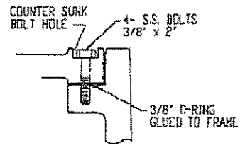
TYPICAL WATERTIGHT DETAIL
