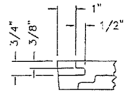
PICKHOLE DETAIL QUARTER SCALE
