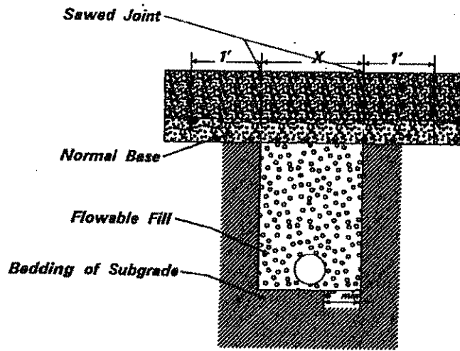
CONCRETE PAVING
