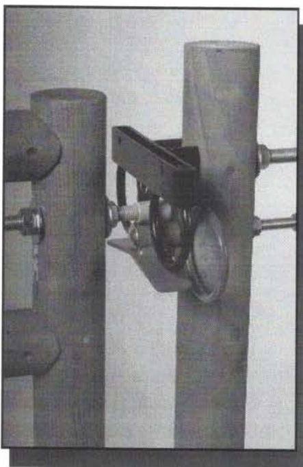
Figure 2—An Accessible Ring Latch with a guard ring (red) on one side.
