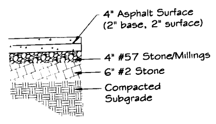
Pavement Detail
