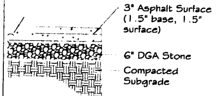
Pavement Detail
