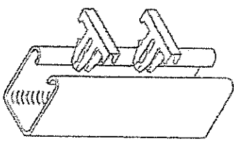
ISOMETRIC EXPLODED VIEW OF ROLL FORM POST AND CLIPS
