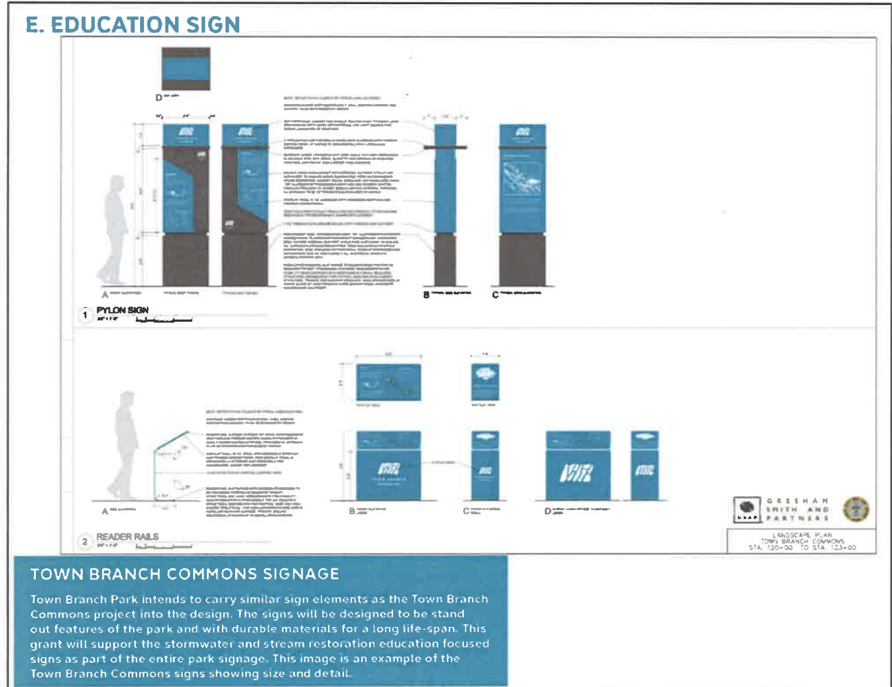
FIGURE 3 – CONCEPTUAL DRAWING OF EDUCATIONAL SIGNAGE (FROM APPLICATION)
