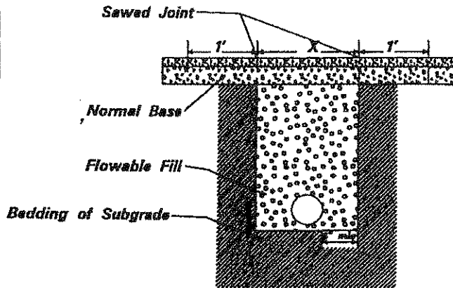
BITUMINOUS PAVING
