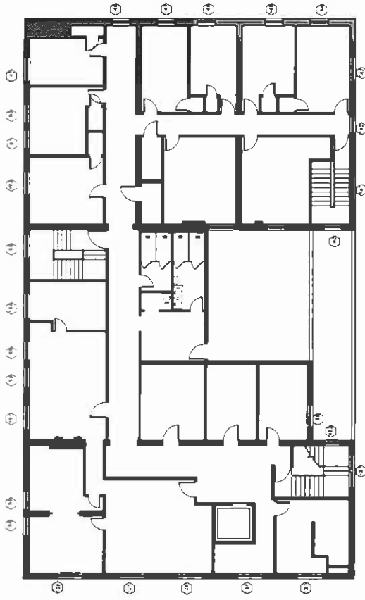
1. FOURTH FLOOR PLAN SCALE 1/8" = 1'-0"
