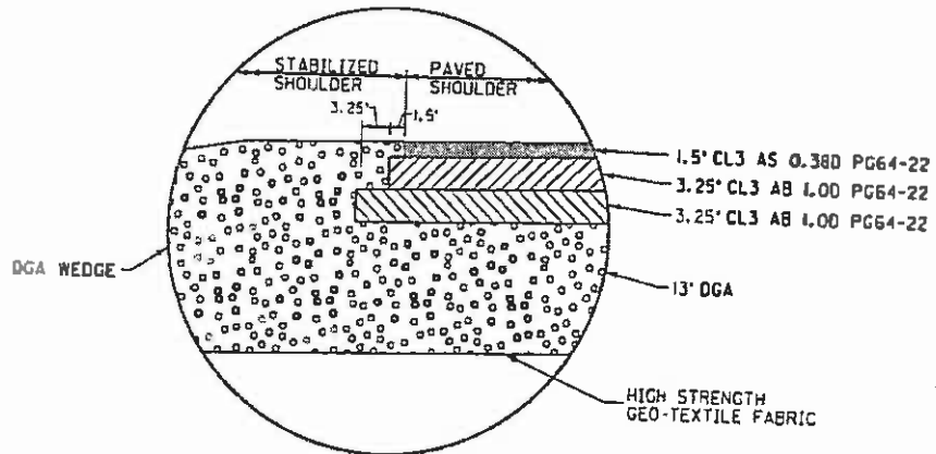
DETAIL "S" NOT TO SCALE
