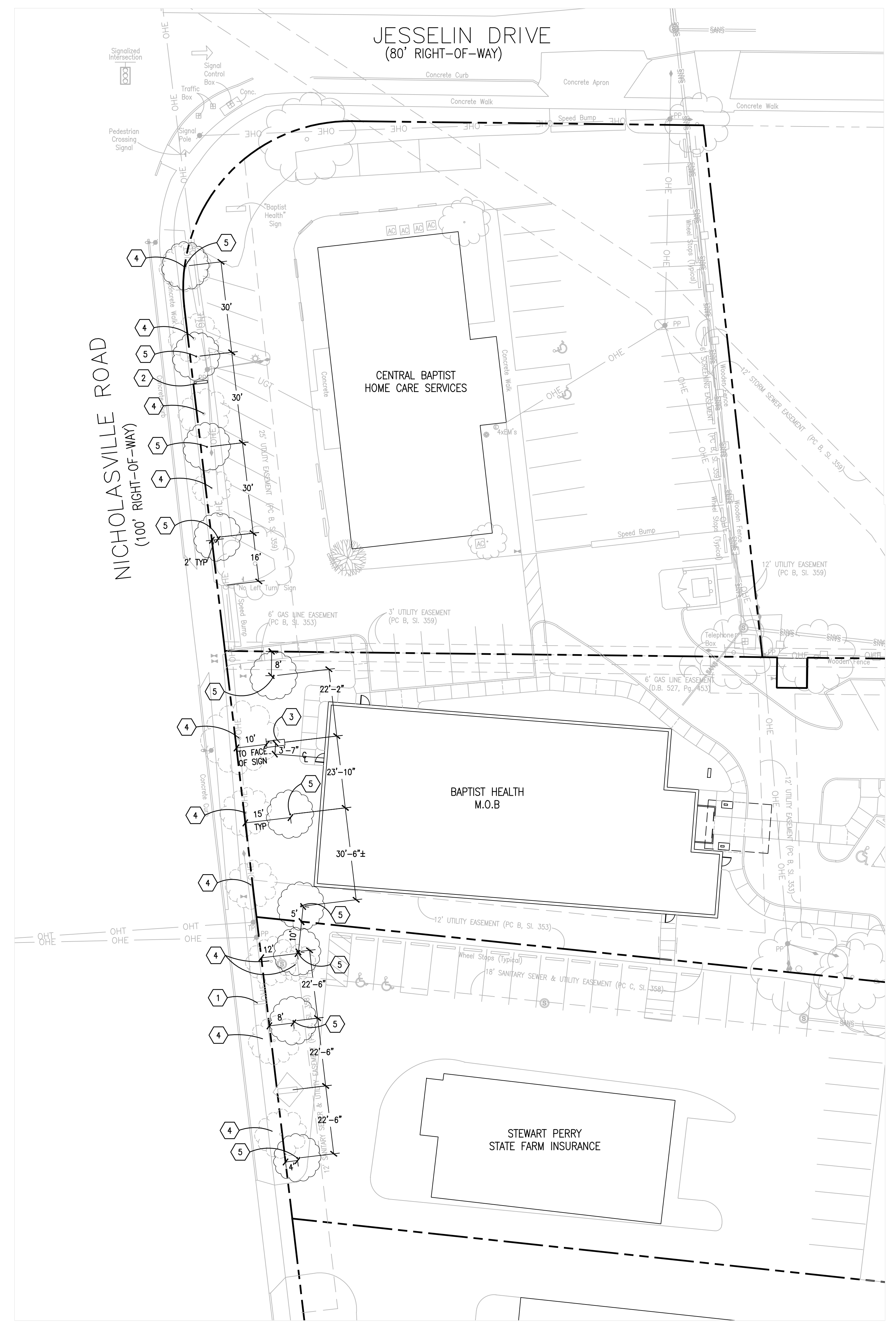
(A) NICHOLASVILLE ROAD CORRIDOR PLAN 1" = 20'
