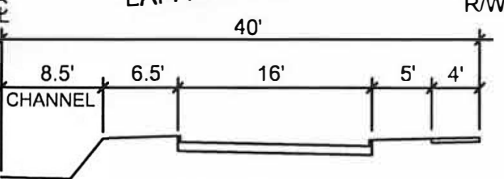
SECTION "B"-"B" SOUTHBEND DRIVE HALF SECTION
