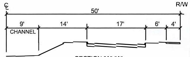
SECTION "A"-"A" LAFAYETTE PKWY HALF SECTION
